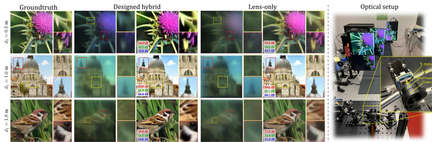
Fig. 3. Three monitor imaging setup using the designed hybrid meta-optics The first column shows examples of the displayed ground truth at distances of d_1 = 0.5, 1.0 , and 1.8 m from top to bottom row, respectively. Specific details of the images are highlighted and shown as zoomed-in sections next to the image. Columns 2 and 3 show the imaging results obtained with the hybrid and lens-only systems, with raw captures and computationally reconstructed images shown left and right, respectively. The PSNR values are reported for each depth and color channel separately and shown as inset in the reconstructed images. The optical setup used for image capture is shown on the very right of the figure. The inset shows an enlarged view of the hybrid camera, consisting of the refractive lens placed at the focal length of 5 mm in front of the sensor and the meta-optics placed directly in front of the refractive lens.
