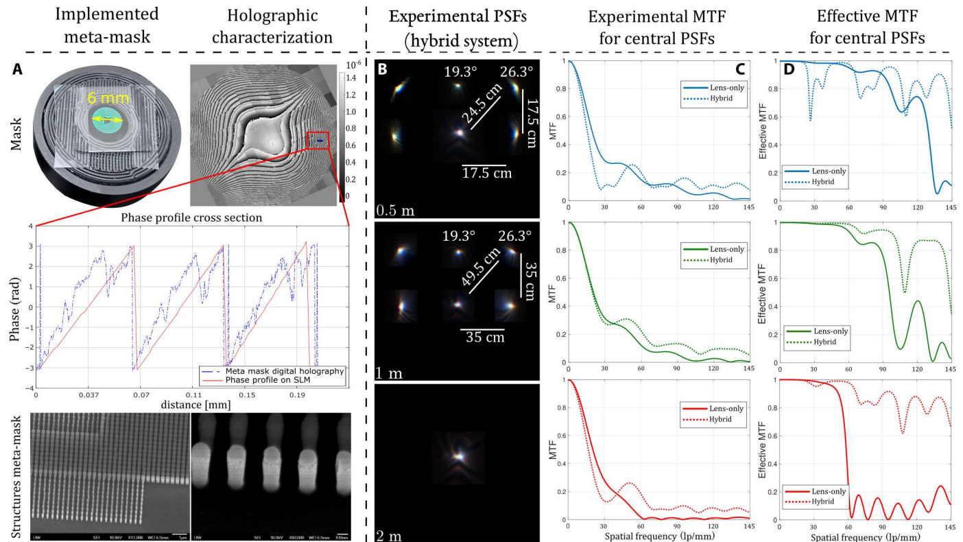
Fig. 2. Holographic characterization of the meta-mask phase profile along with its PSFs across depths and MTFs per channels. (A) Properties of the fabricated meta-optics showing a photograph of the meta-mask on a 3D-printed mount. The bottom row shows scanning electron micrographs highlighting the structural integrity across the device. To determine the quality of the implemented phase, we perform a holographic characterization of the meta-optic, indicating a close match between design (red curve) and measurement (blue). (B) Experimental PSFs of the hybrid system for distances d_1 = 0.5, 1.0 , and 2.0 m. (C and D) Experimental and effective MTFs (EMTFs) for central PSFs of hybrid and lens-only systems.
